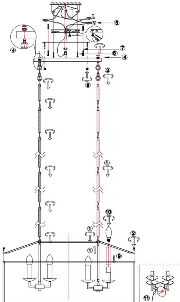
Wire Connection Diagram:
