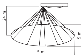
Ceiling Mount sensor Detection Range
